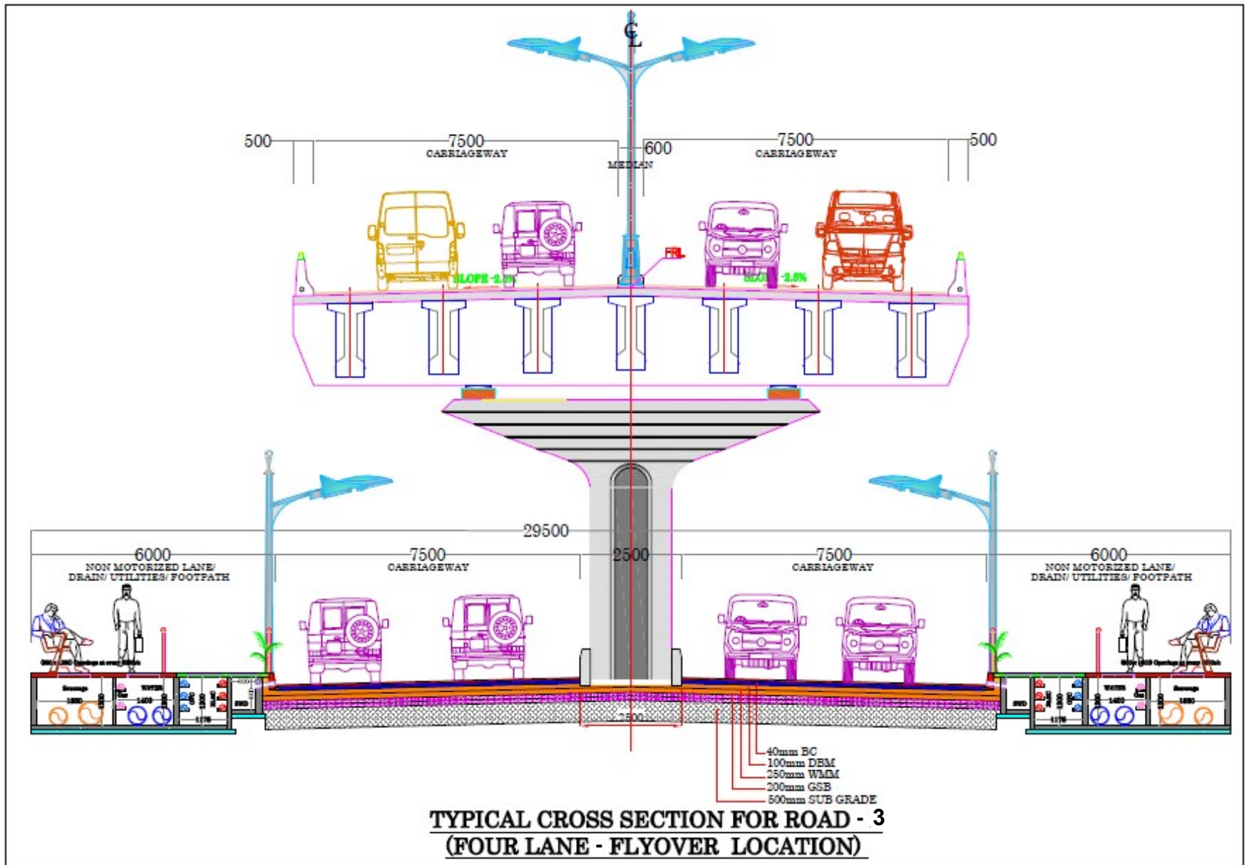
KANTATOLI FLYOVER
