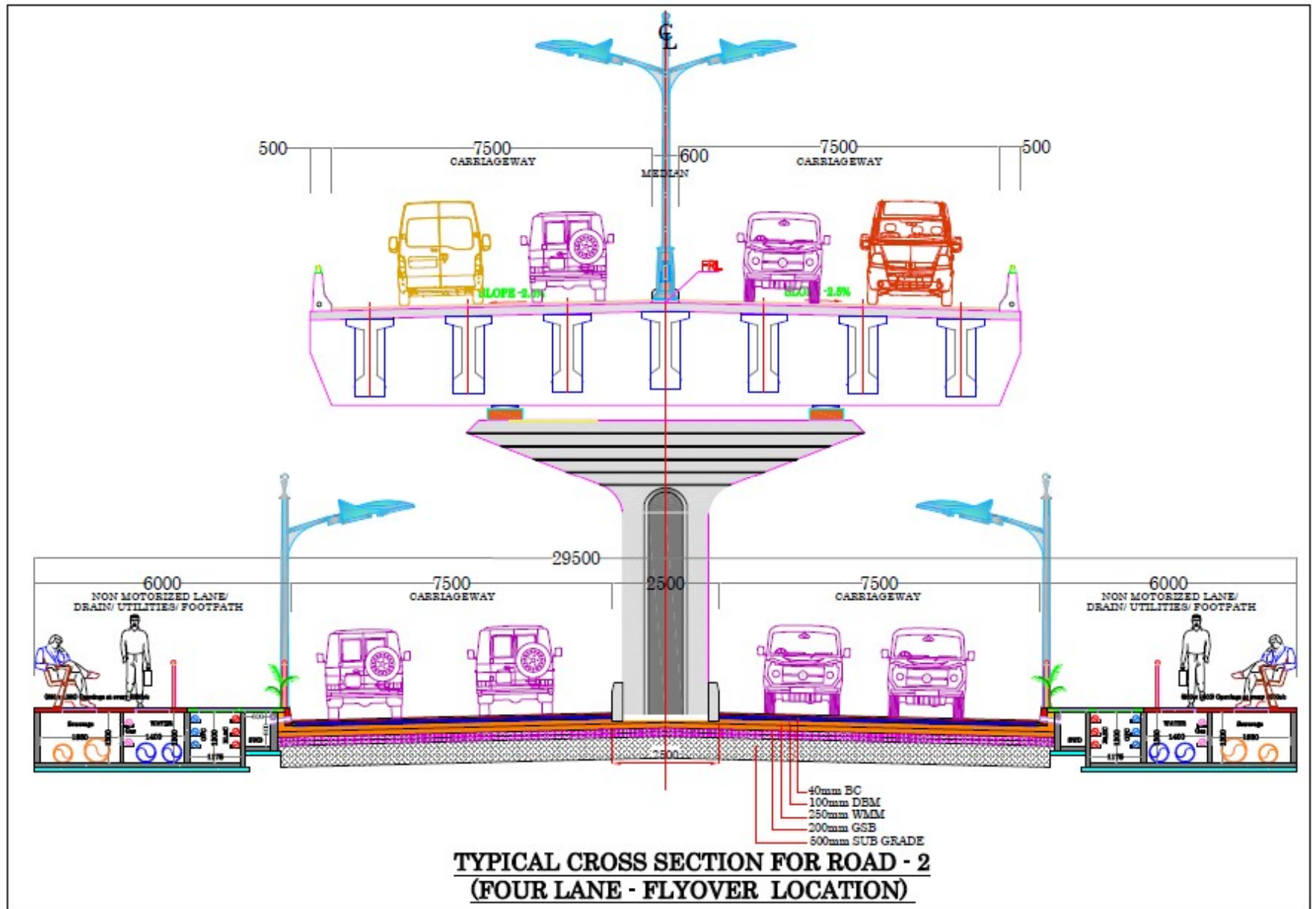
RATU ROAD FLYOVER
